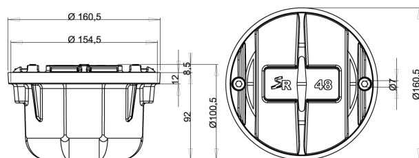
Dimensions: mm
