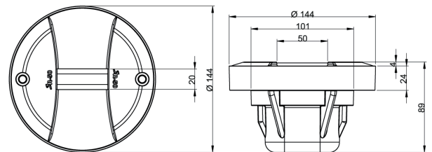
Dimensions: mm
